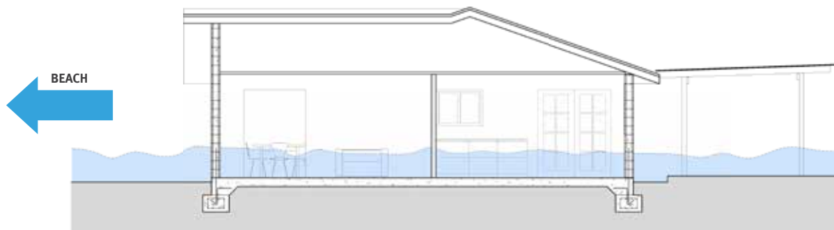
Single storey flow through design for Exposure W homes
