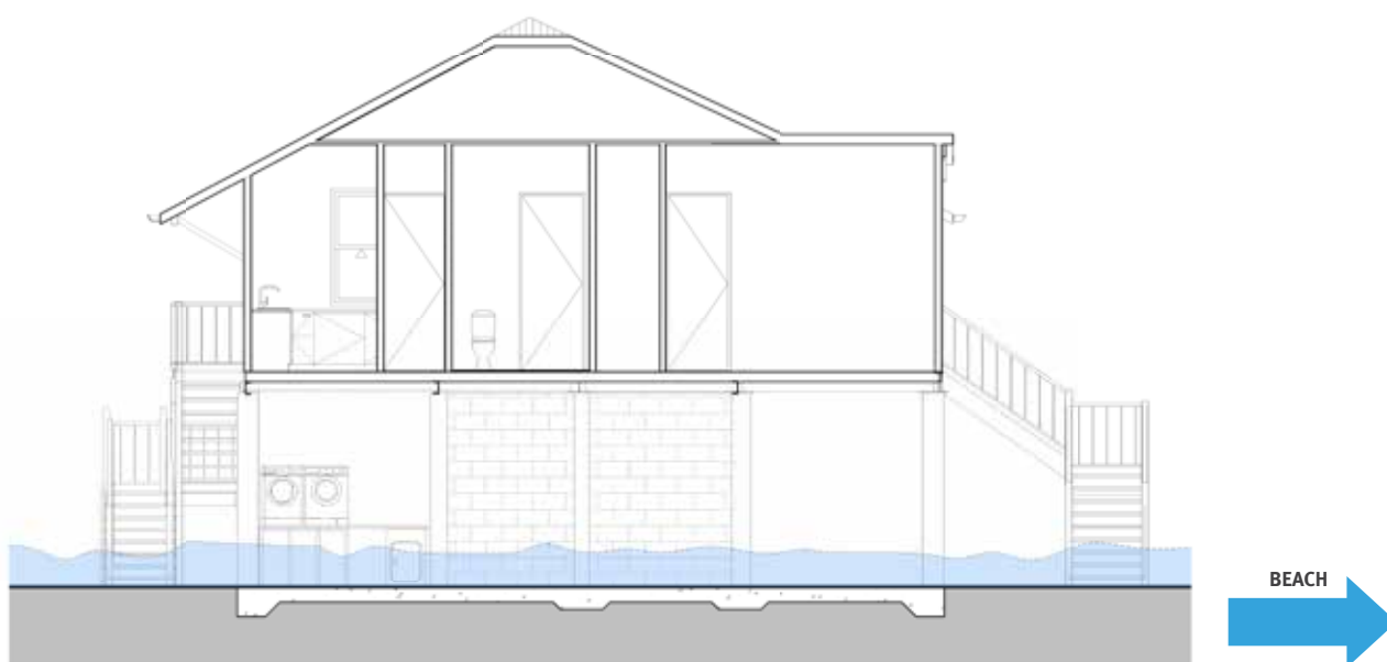
Design for clear flow of water under a high-set home
