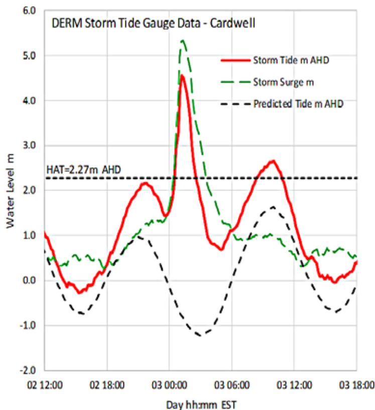
Reconstructed Yasi storm tide event based on the Cardwell tide gauge
